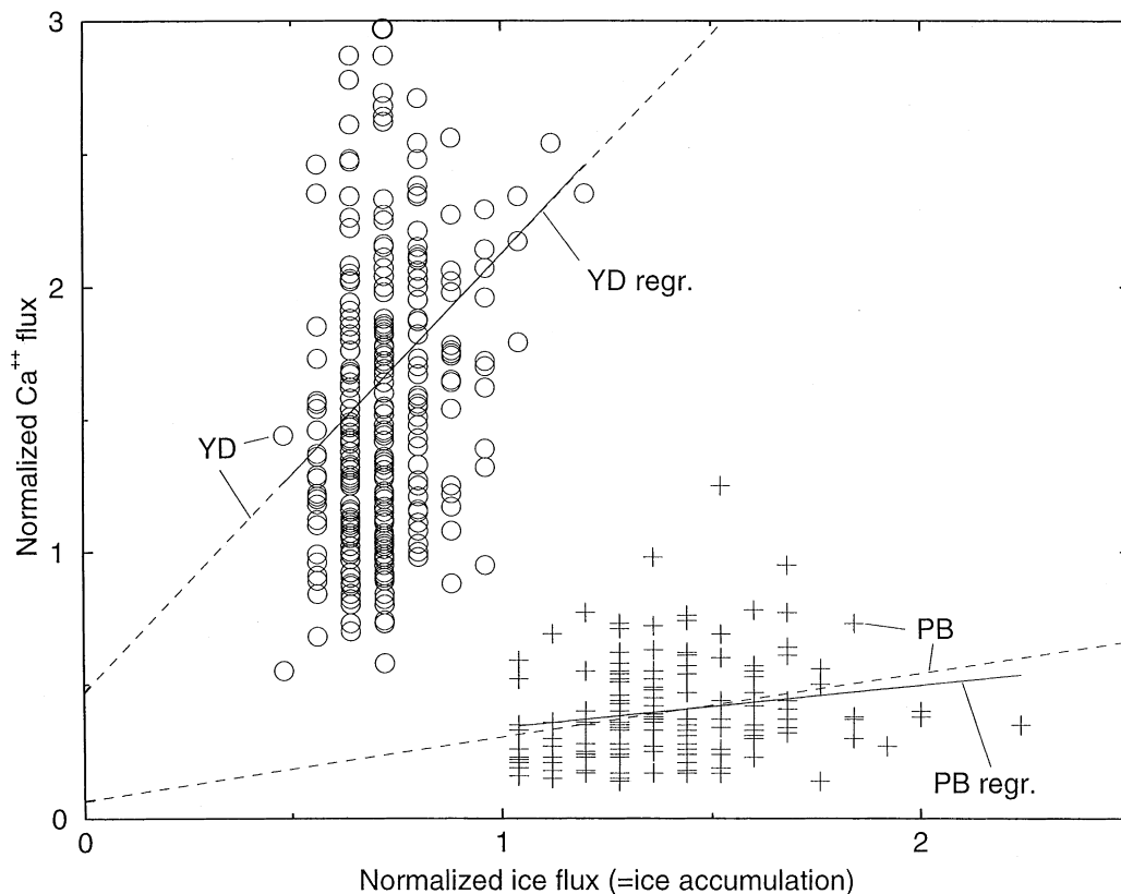
Fig. 2. Comparison of calcium flux to ice flux (snow accumulation rate) for the GISP2 ice core, modified from Alley et al. (1995), with the calcium data from Mayewski et al. (1994, 1997). The data have been normalized by their average values between 11,322 and 14,035 abp. The data sets shown represent 11,322–11,637 abp (during the Preboreal, labeled PB) and 11,759–12,854 abp (Younger Dryas, labeled YD). Solid line segments are individual linear regressions for the YD and for the PB data; dashed lines represent a joint inversion that requires the ratio of the slopes of the lines through the data from the two times to equal the ratio of the intercepts, as hypothesized in the atmospheric-removal model. That ratio is 6.95 in this case, indicating a sevenfold change of calcium loading in the atmosphere sampled by snow accumulation between the Younger Dryas and the few centuries following it (Alley et al., 1995).
