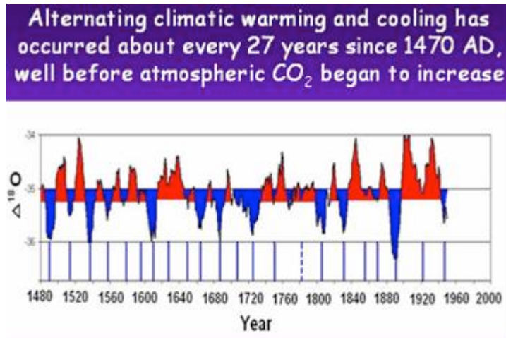
Figure 3. Alternating warm and cool cycles since 1470 AD. Blue = cool, red = warm. Based on oxygen isotope ratios from the GISP2 Greenland ice core.
