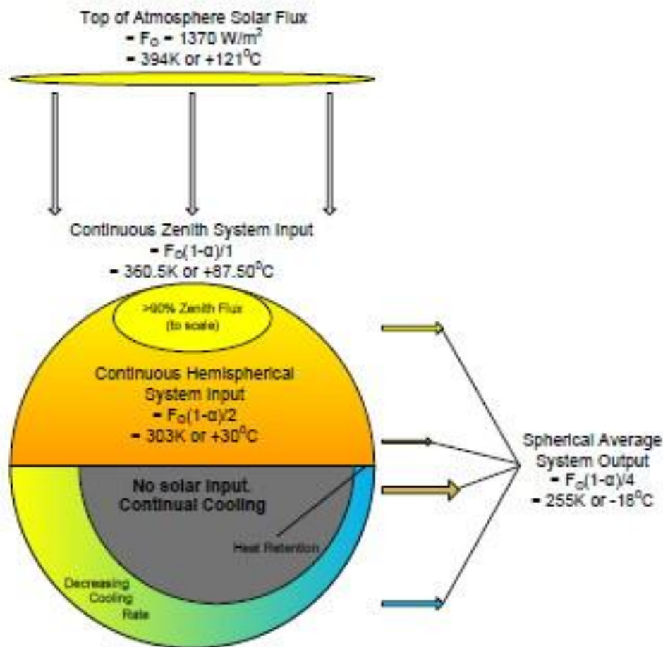
Figure 6: "Outside the System" view of the radiative interaction. Earth is in fact, on average, cooler than the solar radiative input temperature. With this single physical reality, the need to postulate a radiative greenhouse effect evaporates. Image credit: J.E.P.
