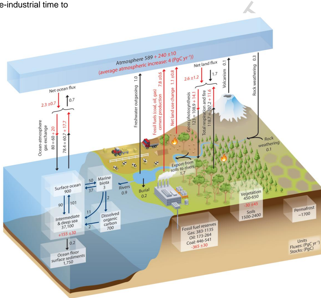
Fig. 1: Simplified schematic of the global carbon cycle. Black numbers and arrows indicate reservoir mass in PgC and exchange in PgC/yr before the Industrial Era. Red arrows and numbers show annual 'anthropogenic' flux changes averaged over the 2000–2009 time period. Graphic from AR5-Chap.6-Fig.6.1 .
